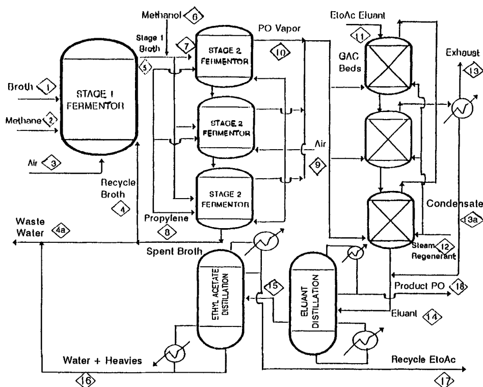
Fig. 1. Schematic of the conventional process of methanotrophic oxidation.
